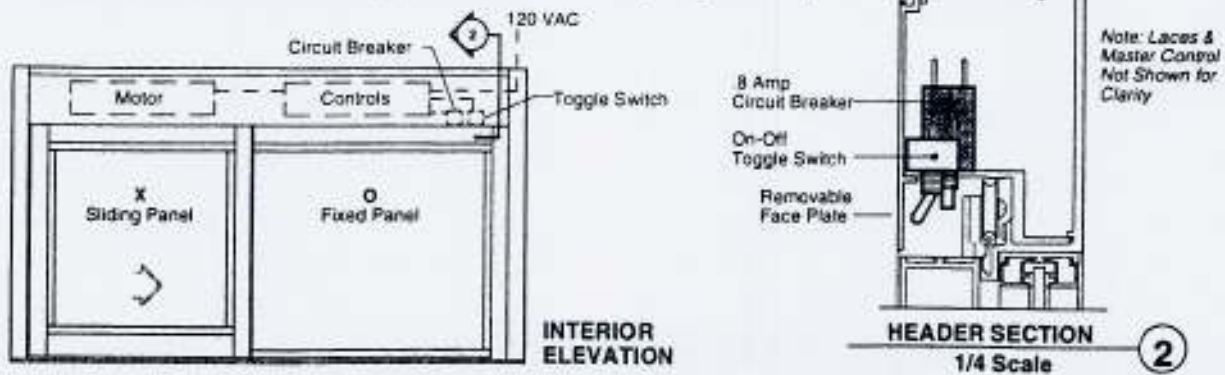
Fig. 8 - Circuit Breaker & On-Off Toggle Switch Location ( Single Slide )
