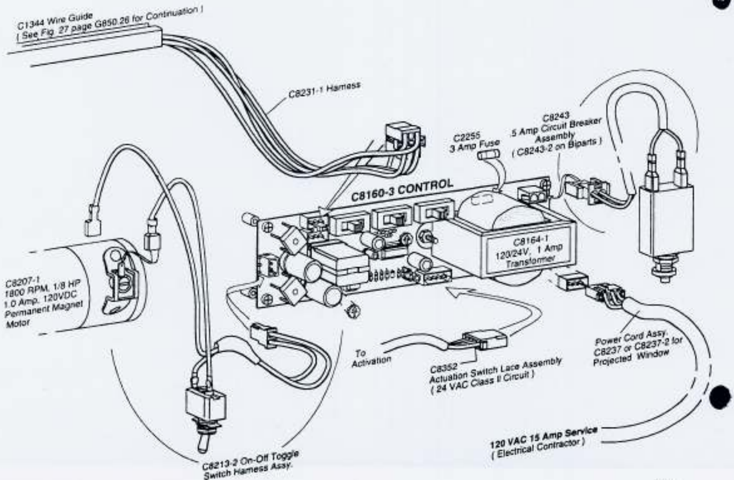
Fig. 5 - C8160-3 Master Control and Connections
