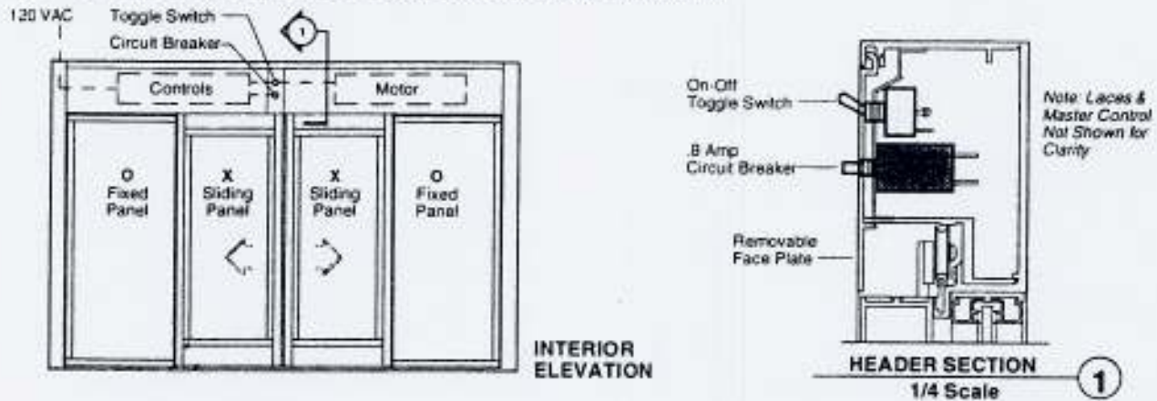
Fig. 7 - Circuit Breaker & On-Off Toggle Switch Location ( Bipart )
