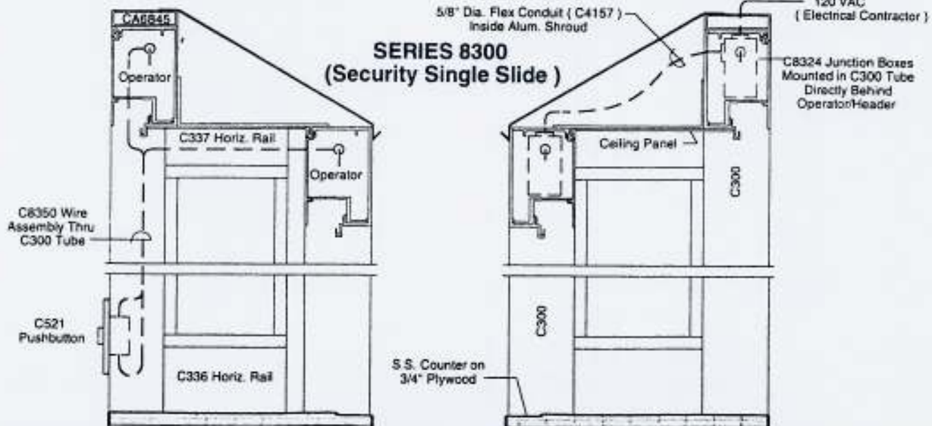
SECTION - Interior Left Side
