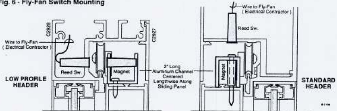
Fig. 6 - Fly-Fan Switch Mounting
