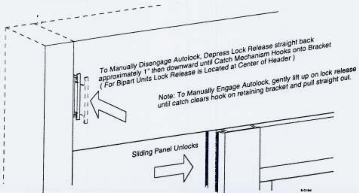
Fig. 4 - Manual Autolock Release
