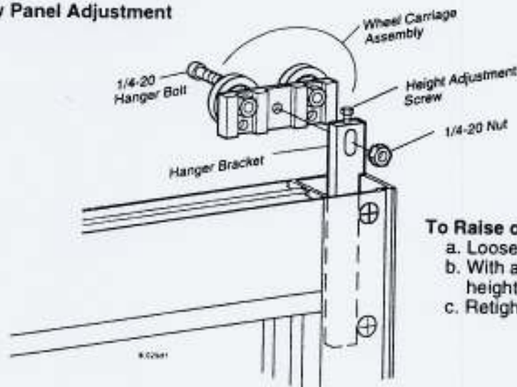
Fig. 21 - Window Panel Adjustment
