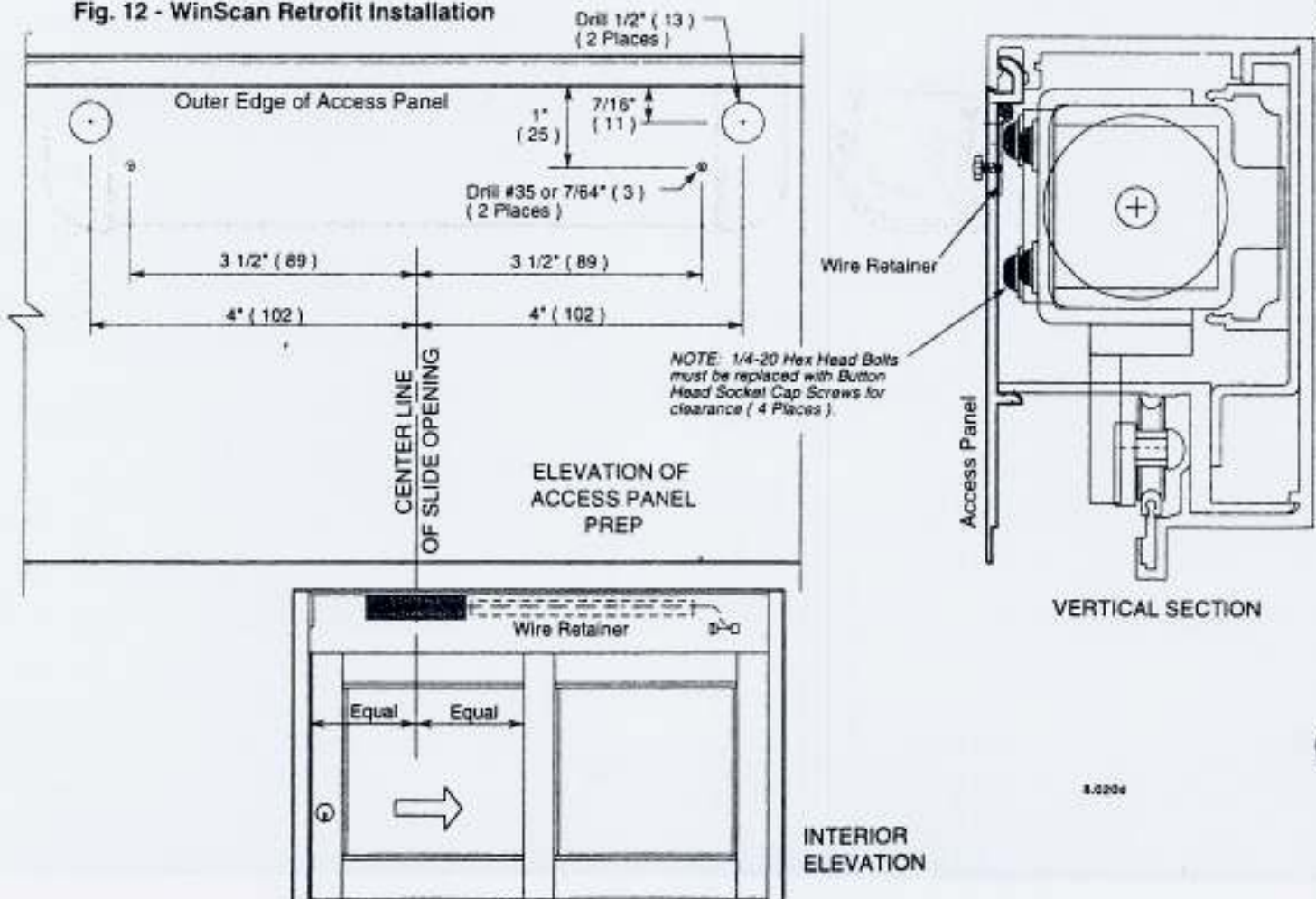
Fig. 12 - WinScan Retrofit Installation
