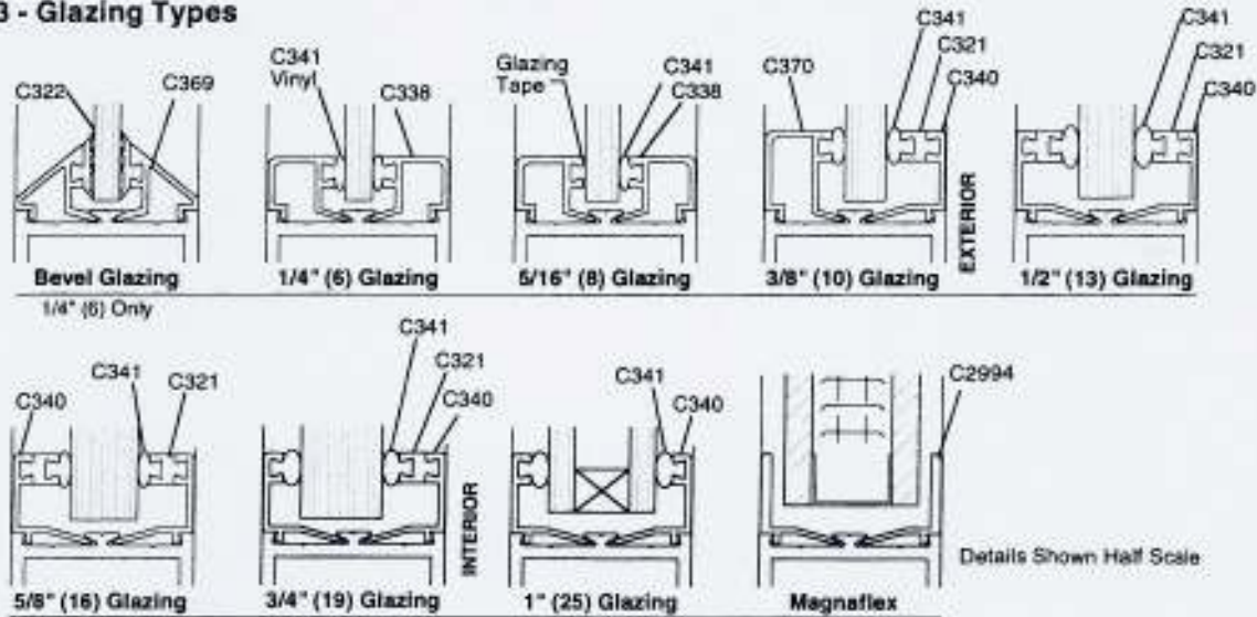
Figure 23 - Glazing Types
