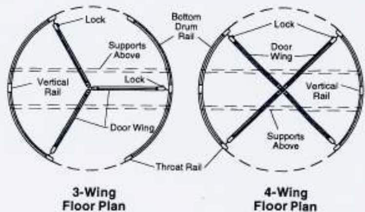
Figure 1 - Plan View of Round Revolving Doors
