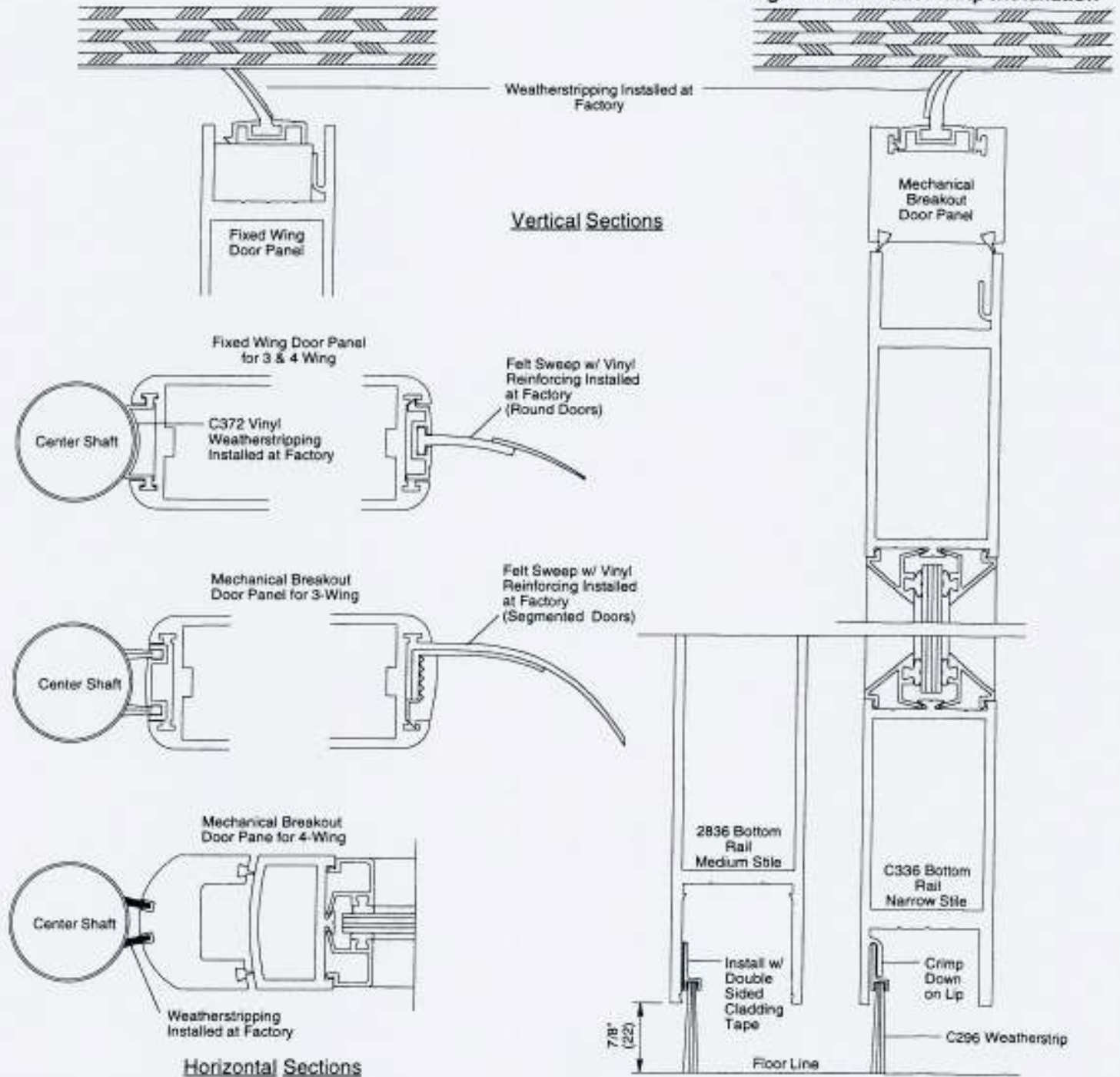
Figure 12 - Weatherstrip Installation
