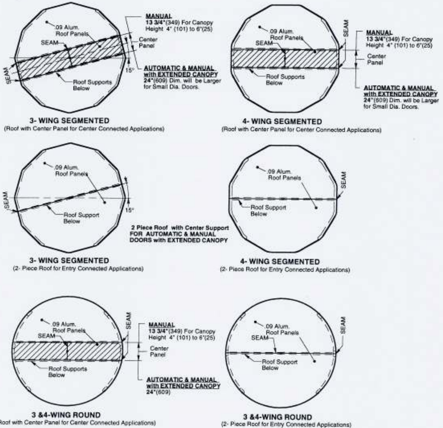
Figure 27 - Roof Plans
