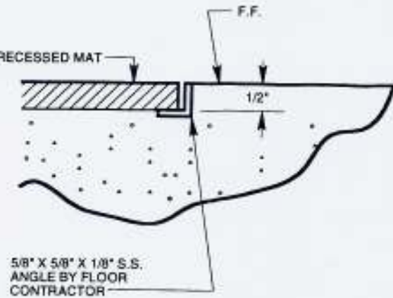
Figure 29 - Recessed Mat
