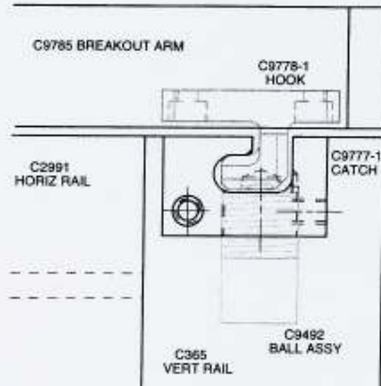
Figure 20 - Side View At Ball Catch
