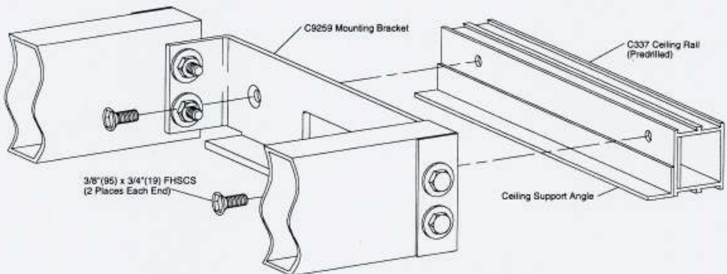
Figure 5 - Support Tube Assembly Installation (Segmented Revolver)
