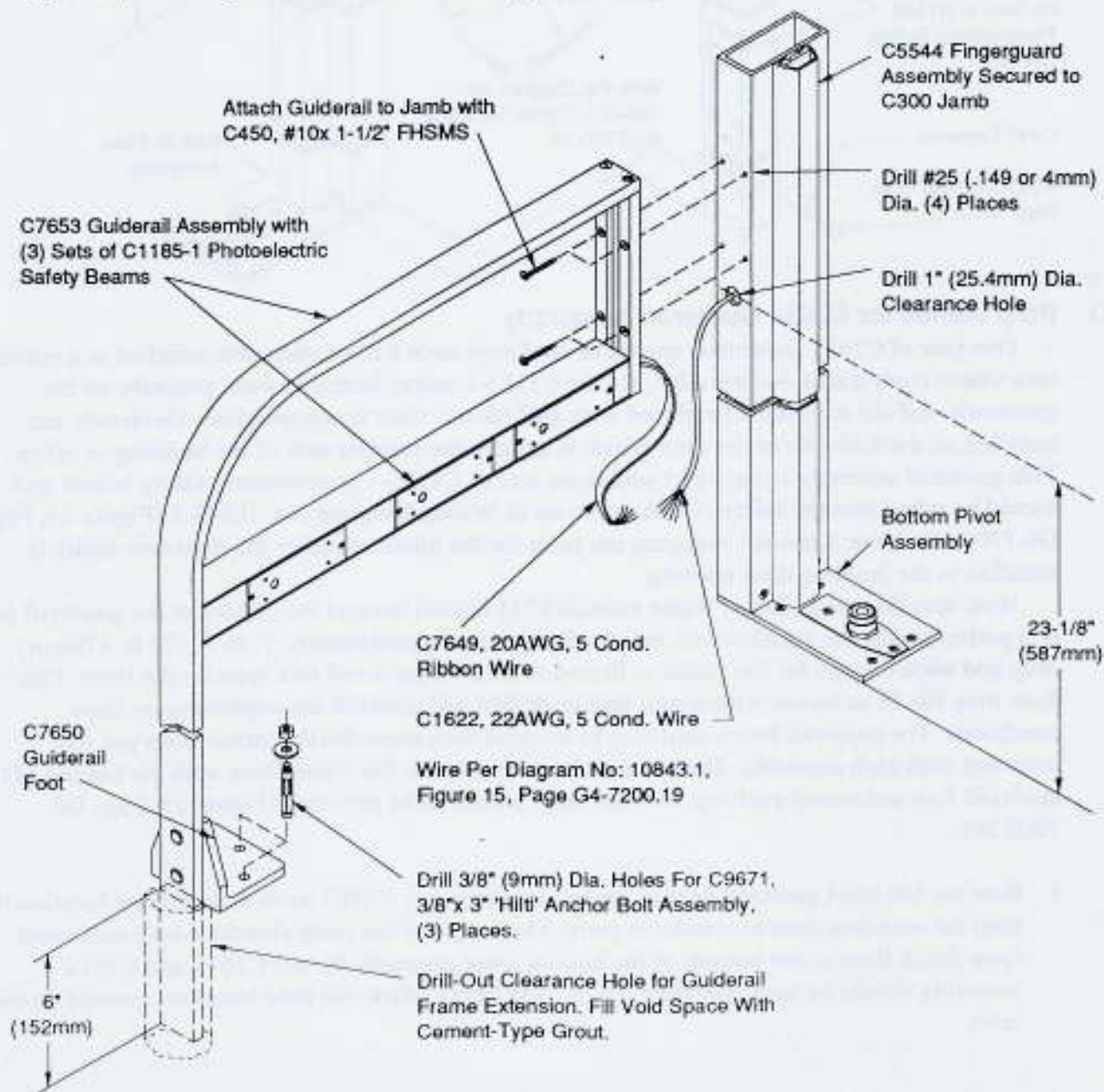
Figure 23, Attaching C7653 Guiderail Assembly to C300 Jamb
