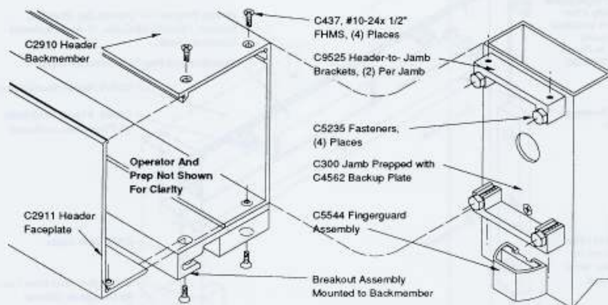
Figure 25, Attaching Header to Jambs
