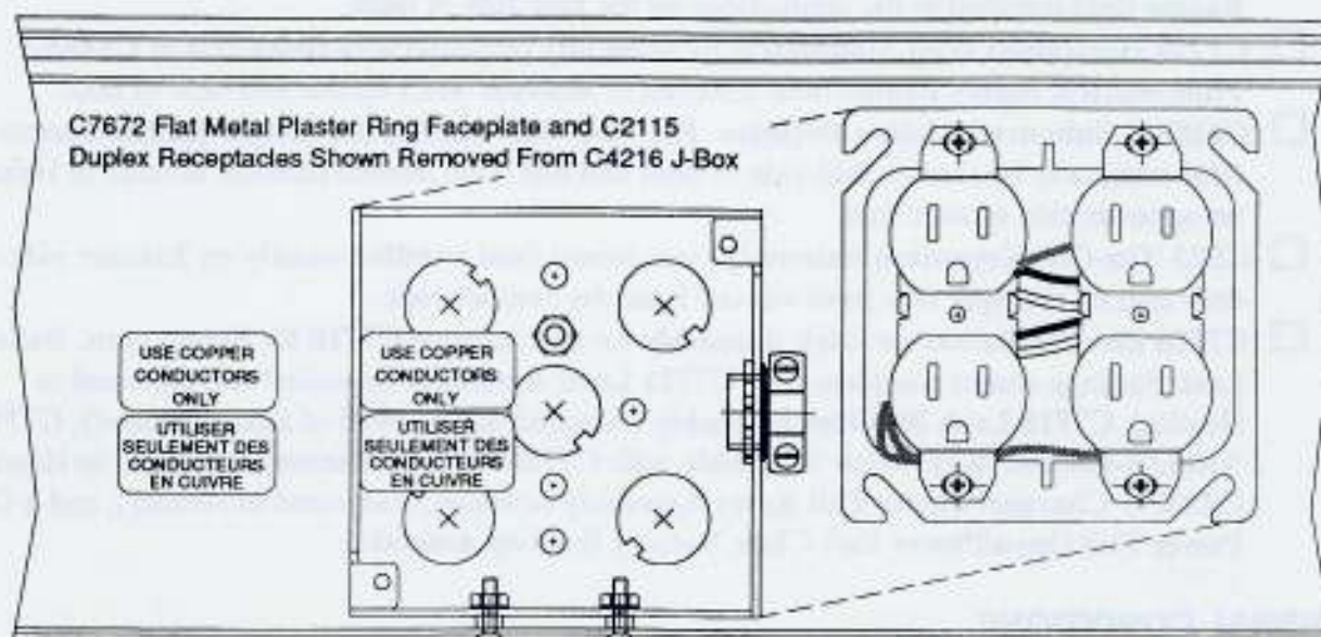
Figure 10, Front View of C7671 Quadplex Junction Box Assembly
