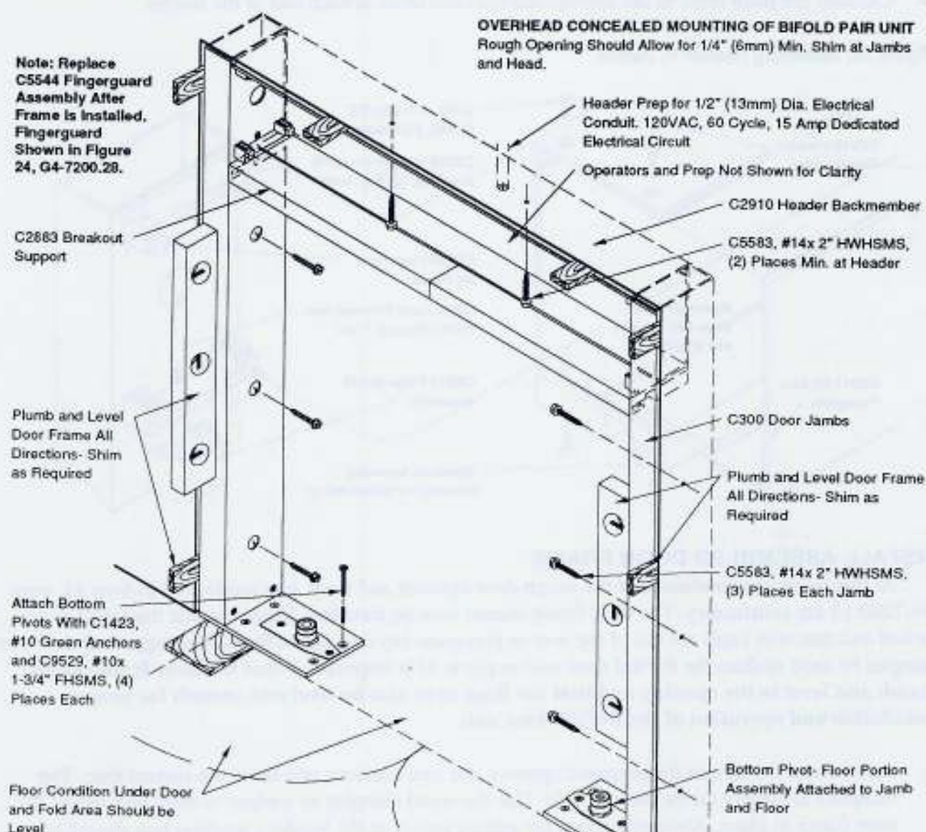
Figure 26, Installing Assembled Door Frame
