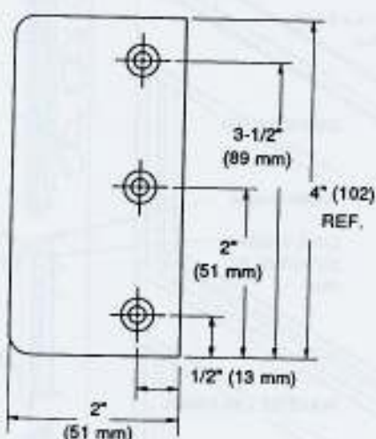
Figure 27, Installing C7641-1 Pull Handle Assembly
