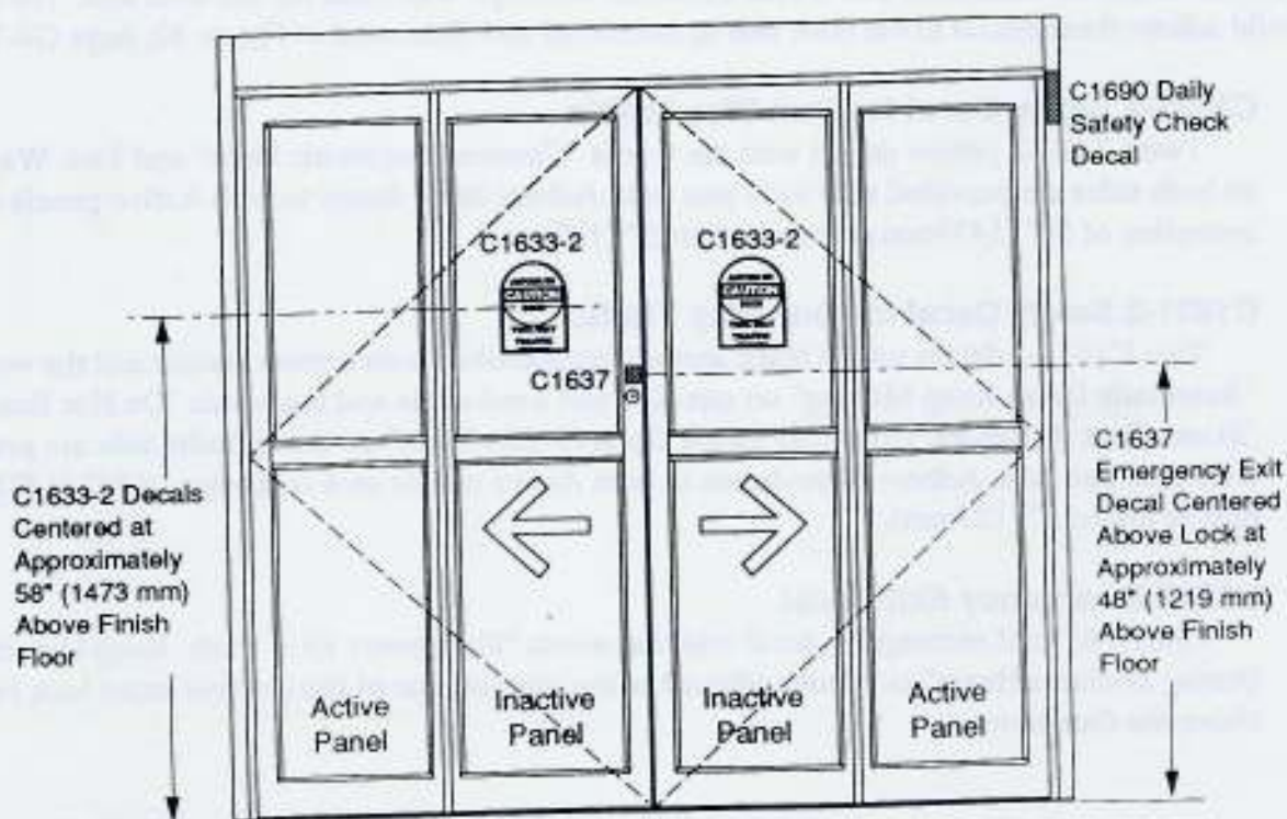
INTERIOR VIEW ELEVATION BIFOLD DOOR TYPE: LHR-RHR PAIR
