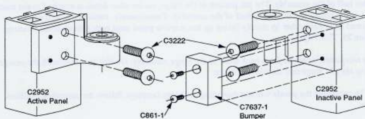
Figure 30, Exploded View of LHR Hinge Assembly
