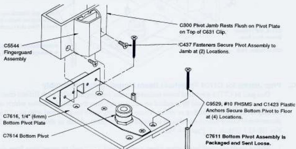
Figure 19, Attaching C7611 Bottom Pivot Assembly to C300 Jamb
