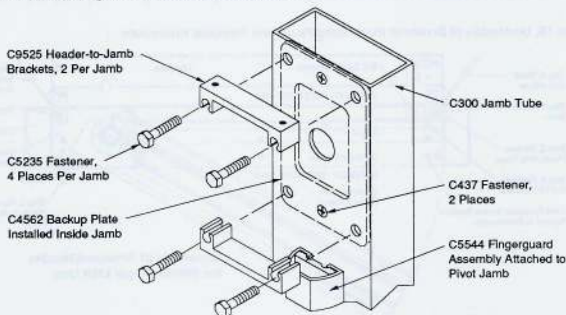
Figure 18, Attaching C9525 Brackets to C300 Jamb
