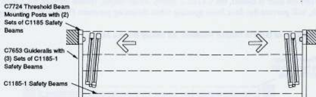
Figure 8, Plan View of Door in Open Position- First Two Gulderall Safety Beams Detect Door, Maintain Hold-Open Function
