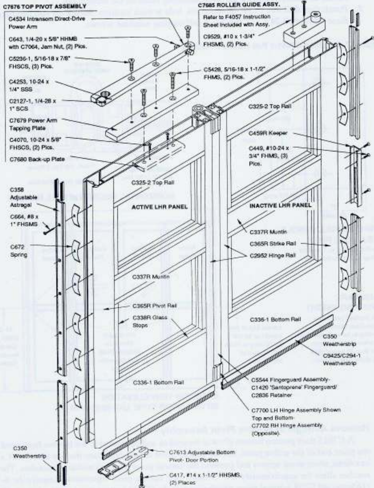
Figure 28, Exploded View of Active/Inactive Panels
