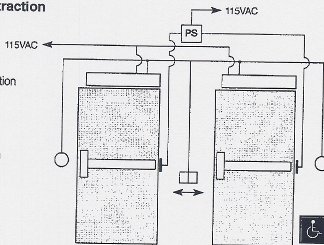
Latch Retraction
