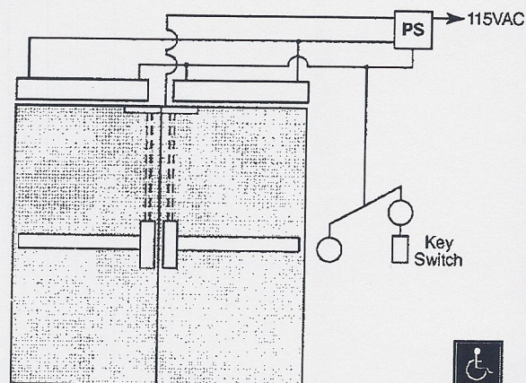
Electric Strikes
