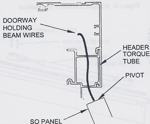
Figure 7. Installing the SO Panel
