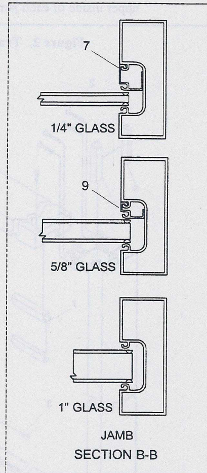
Figure 2. Transom Assembly (Sheet 2 of 2)
