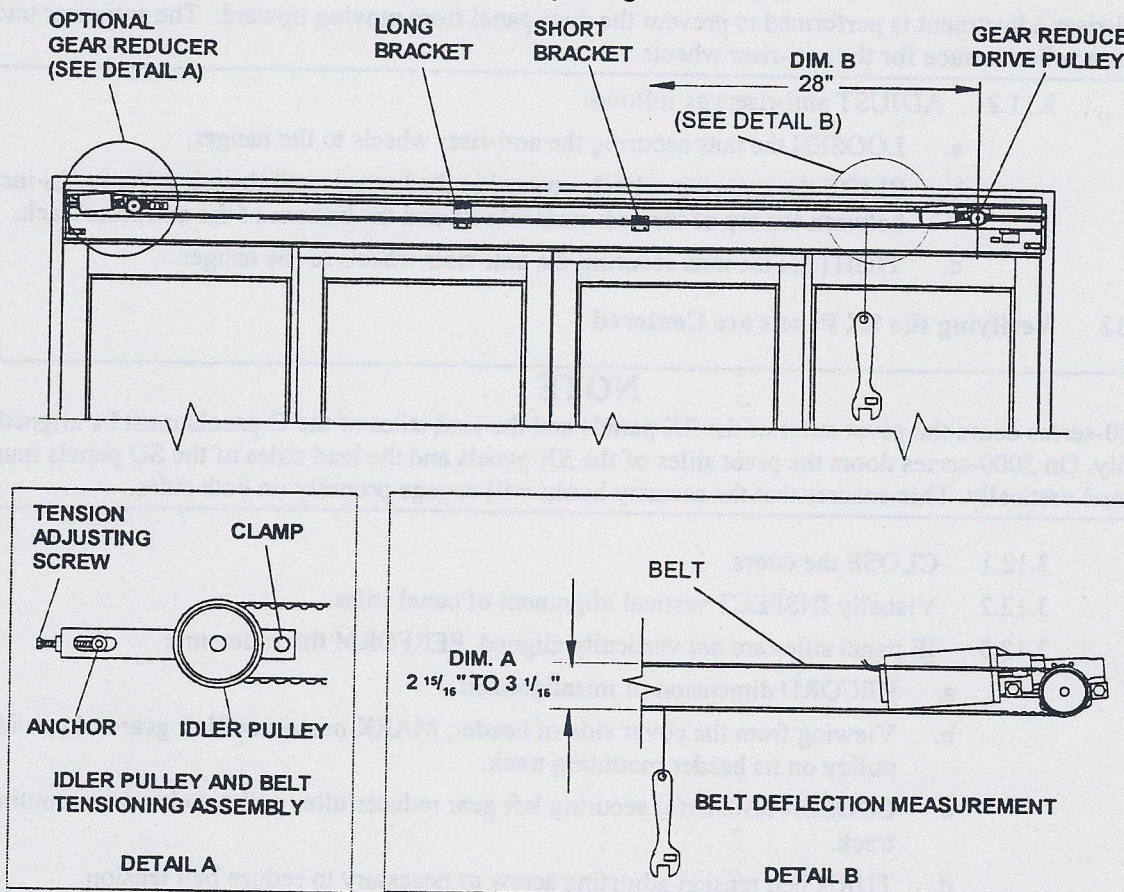
Figure 12. Adjusting Belt Tension
