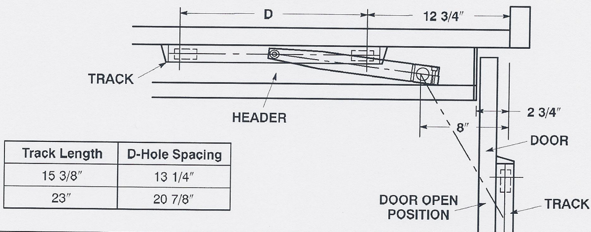
Figure 2. Header Preparation
