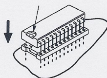
Figure 1. Polarity Indicator
