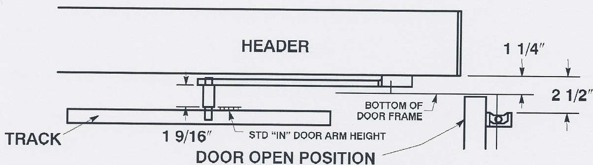
Figure 3. Mounting Hole Locations
