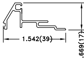
GUTTER-BEVELED EXTRUSION
