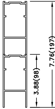
NOMINAL 8"
