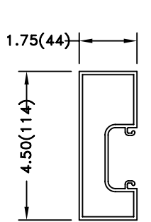
STANDARD JAMB-4 1/2"
