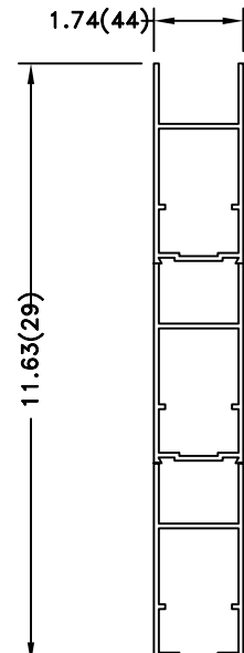
12" NOMINAL MUNTIN BAR
