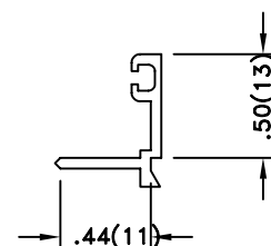
GLASS STOP EXTRUSION
