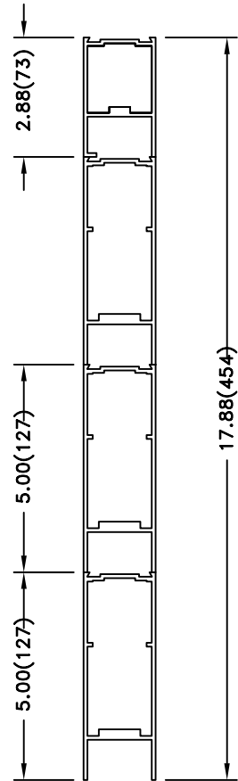
NOMINAL 18"
