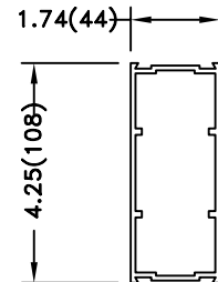
4 1/4" EXTRUSION MUNTIN BAR
