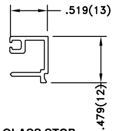
GLASS STOP EXTRUSION
