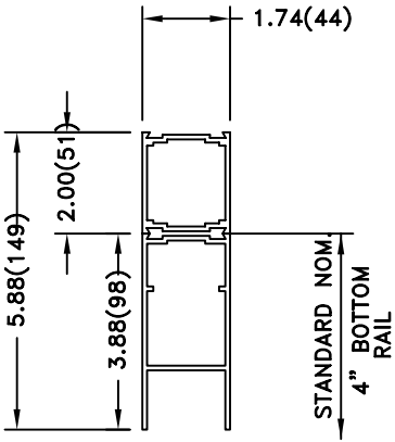
NOMINAL 6"
