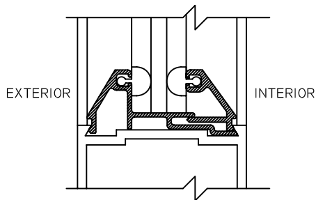
GUTTER-BEVELED EXTRUSION (RUNS HORIZONTALLY)
