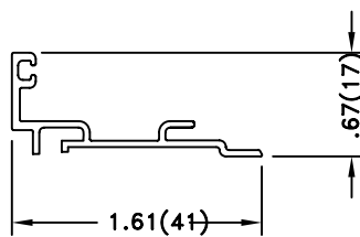
GLASS STOP-GUTTER EXTRUSION
