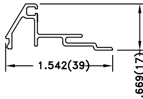
GUTTER-BEVELED EXTRUSION
