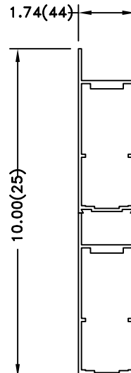
10" NOMINAL MUNTIN BAR
