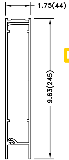
10" SEAMLESS
