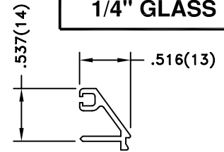
GLASS STOP-BEVELED EXTRUSION
