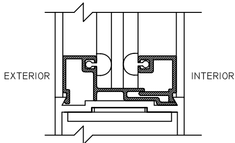
GUTTER EXTRUSION (RUNS VERTICALLY)
